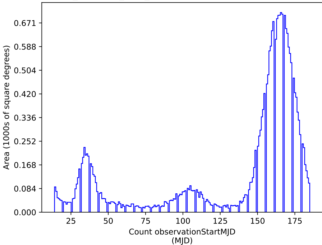
noroll_mjdp120_v3.4_10yrs y: Count observationStartMJD
