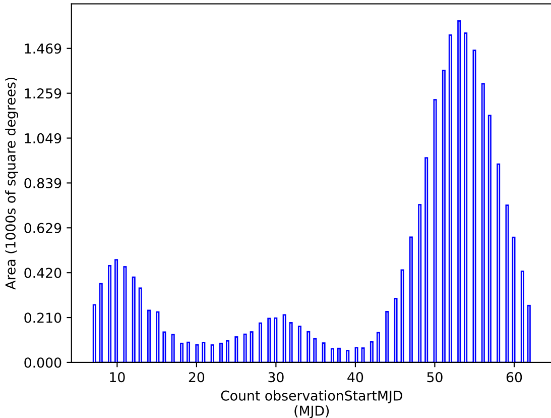
noroll_mjdp120_v3.4_10yrs u: Count observationStartMJD
