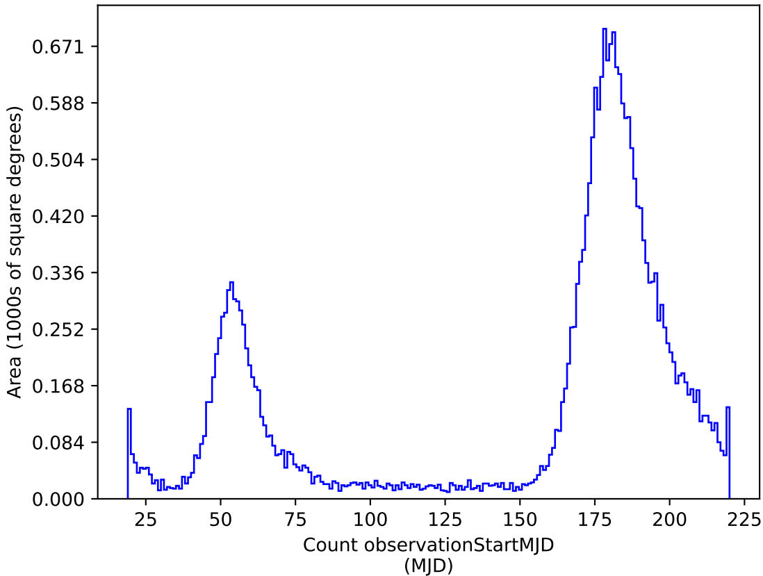
noroll_mjdp120_v3.4_10yrs r: Count observationStartMJD
