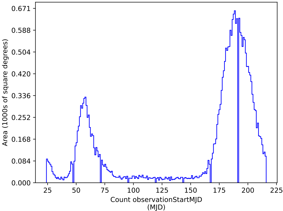
noroll_mjdp120_v3.4_10yrs i: Count observationStartMJD
