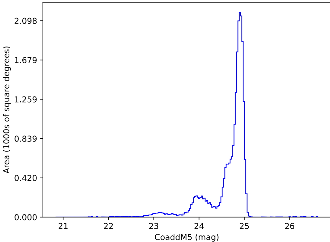
noroll_mjdp120_v3.4_10yrs y: CoaddM5
