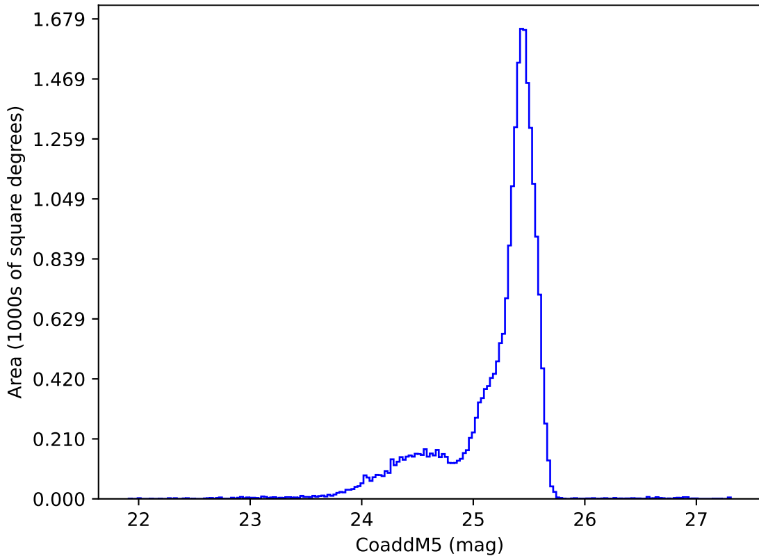
noroll_mjdp120_v3.4_10yrs u: CoaddM5
