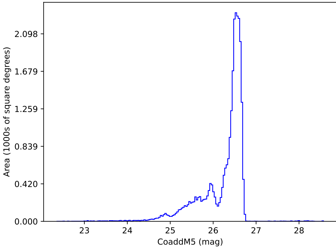
noroll_mjdp120_v3.4_10yrs i: CoaddM5
