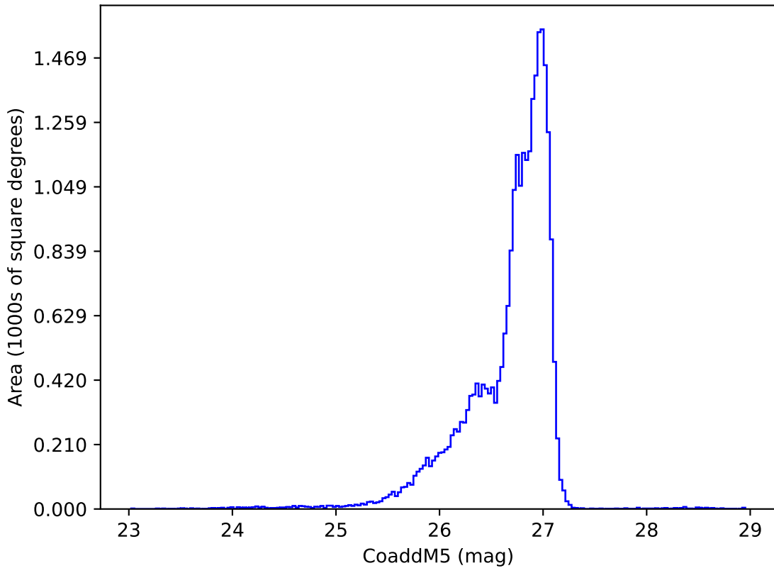
noroll_mjdp120_v3.4_10yrs g: CoaddM5
