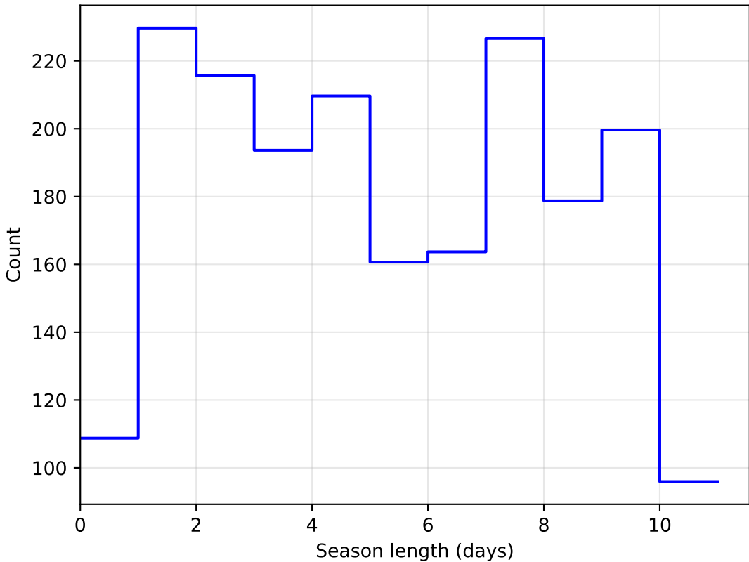
noroll_mjdp120_v3.4_10yrs DD:WFD all bands: SeasonLength
