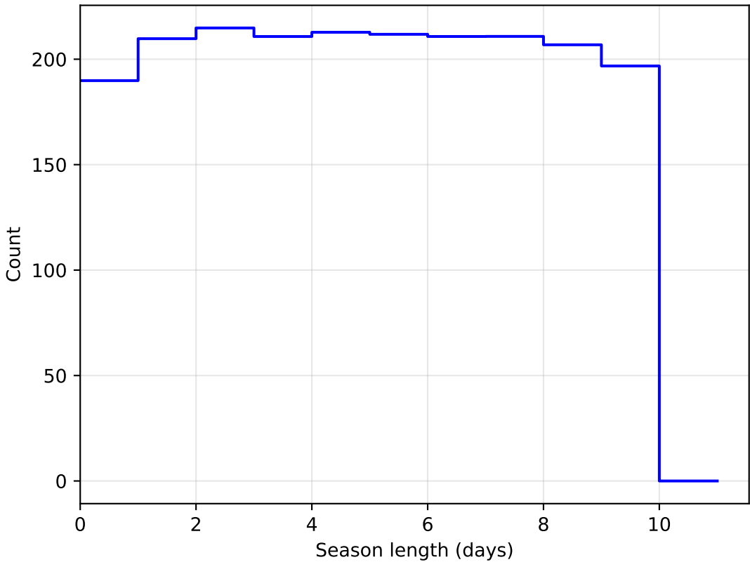
noroll_mjdp120_v3.4_10yrs DD:EDFS all bands: SeasonLength
