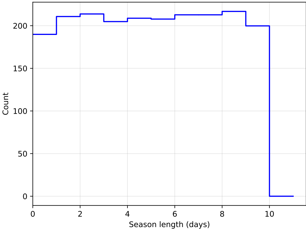
noroll_mjdp120_v3.4_10yrs DD:ECDFS all bands: SeasonLength
