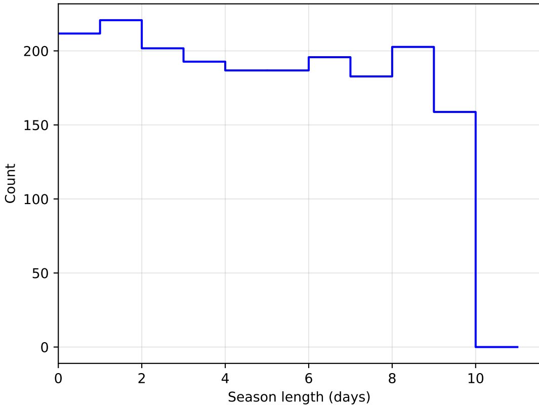
noroll_mjdp120_v3.4_10yrs DD:COSMOS all bands: SeasonLength
