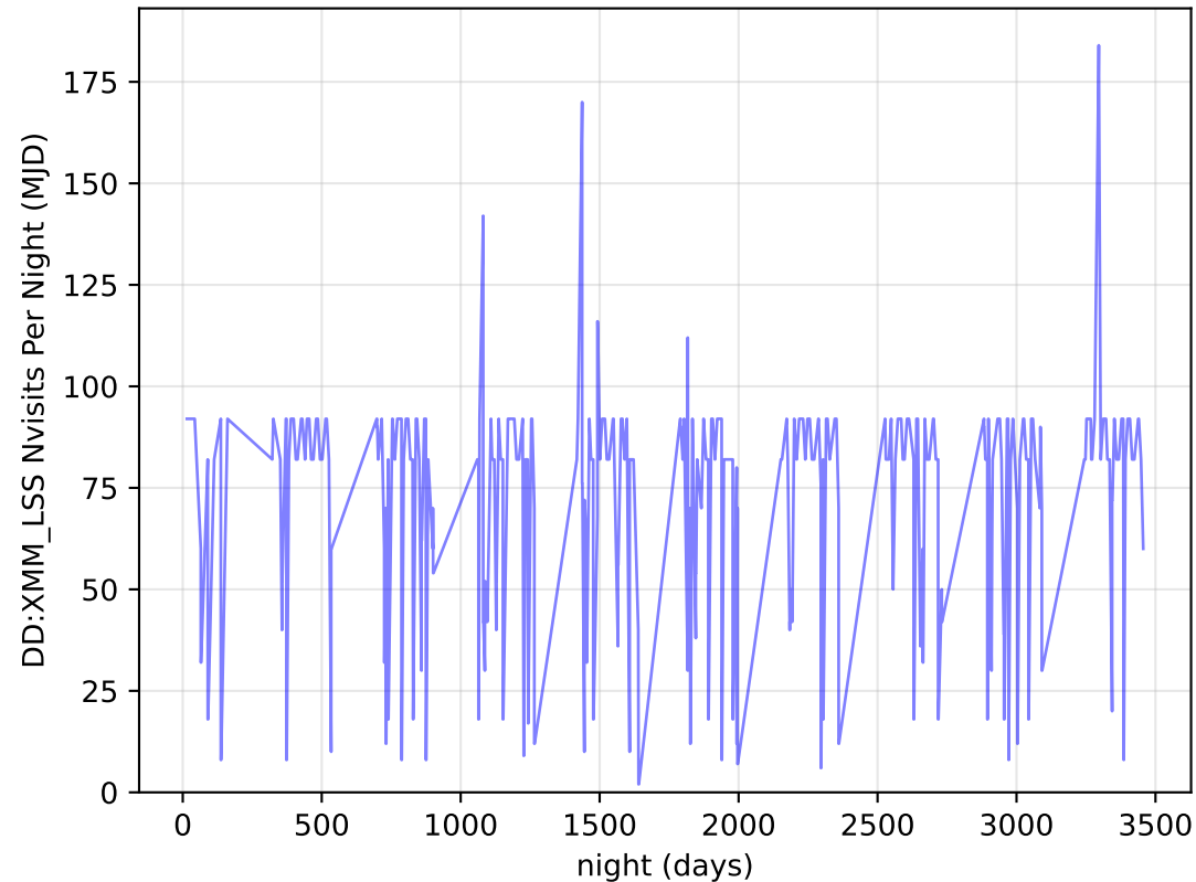
noroll_mjdp120_v3.4_10yrs all bands: DD:XMM_LSS Nvisits Per Night
