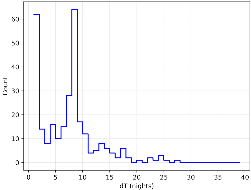
noroll_mjdp120_v3.4_10yrs all bands: DD:XMM_LSS Delta Nights Histogram
