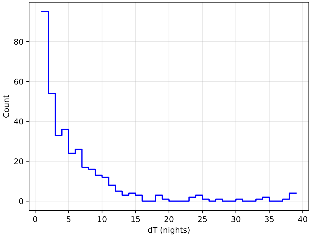
noroll_mjdp120_v3.4_10yrs all bands: DD:WFD Delta Nights Histogram
