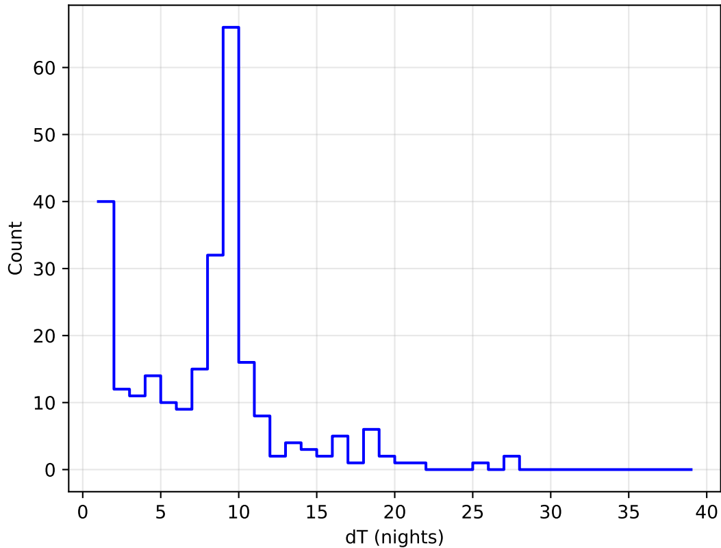
noroll_mjdp120_v3.4_10yrs all bands: DD:ELAISS1 Delta Nights Histogram
