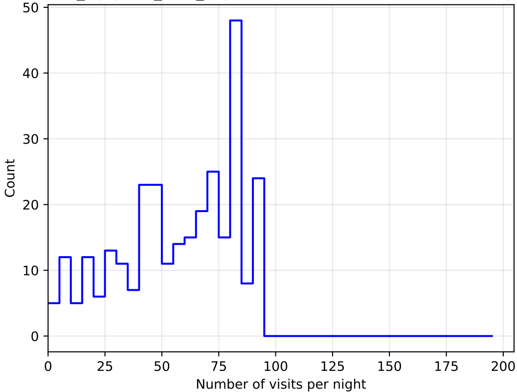
noroll_mjdp120_v3.4_10yrs all bands: DD:EDFS NVisitsPerNight
