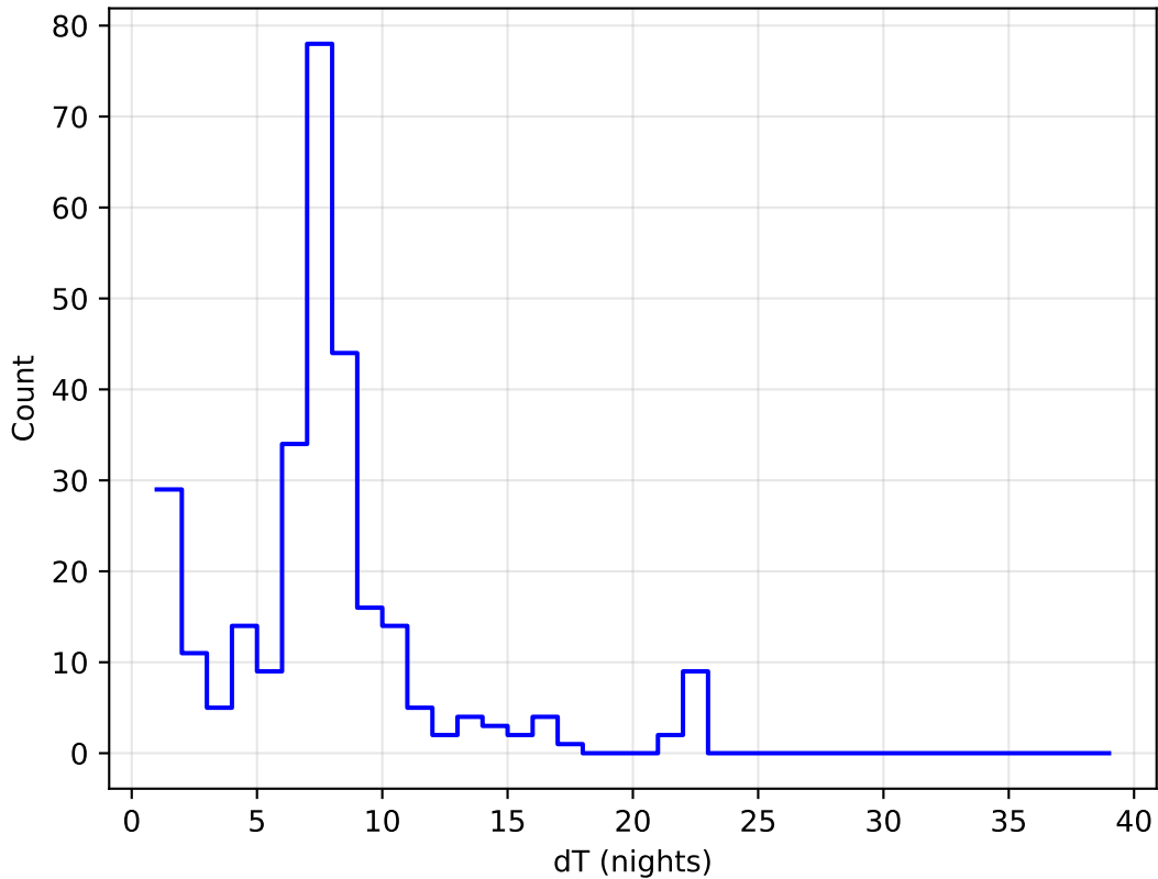
noroll_mjdp120_v3.4_10yrs all bands: DD:EDFS Delta Nights Histogram
