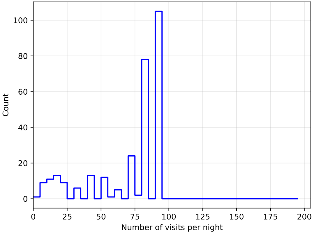
noroll_mjdp120_v3.4_10yrs all bands: DD:ECDFS NVisitsPerNight
