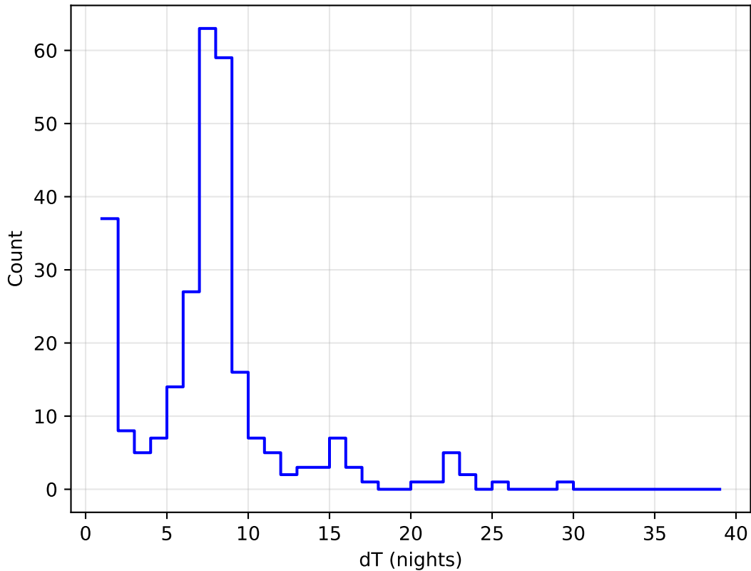
noroll_mjdp120_v3.4_10yrs all bands: DD:ECDFS Delta Nights Histogram
