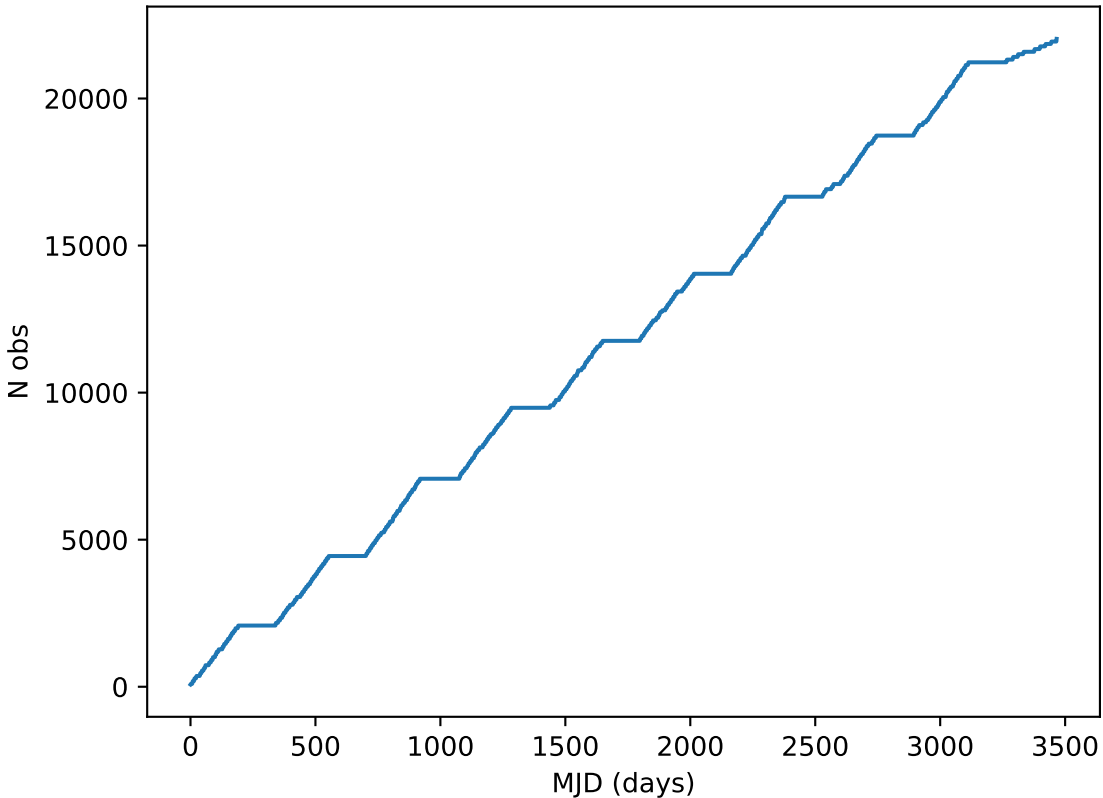
noroll_mjdp120_v3.4_10yrs all bands: DD:ECDFS Cumulative NVisits
