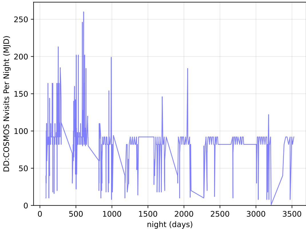
noroll_mjdp120_v3.4_10yrs all bands: DD:COSMOS Nvisits Per Night
