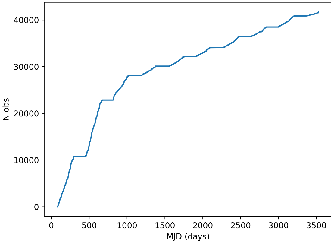
noroll_mjdp120_v3.4_10yrs all bands: DD:COSMOS Cumulative NVisits
