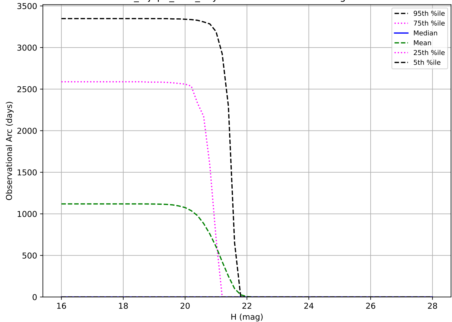
noroll_mjdp0_v3.4_10yrs: Observational Arc Length Vatira
