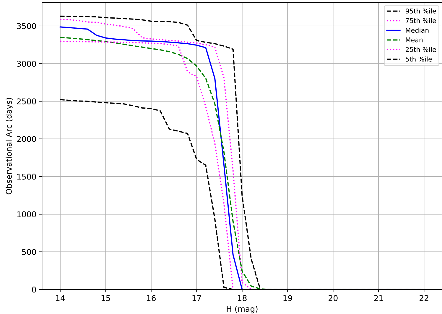
noroll_mjdp0_v3.4_10yrs: Observational Arc Length Trojan
