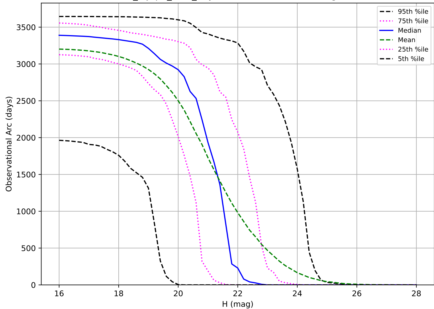
noroll_mjdp0_v3.4_10yrs: Observational Arc Length PHA
