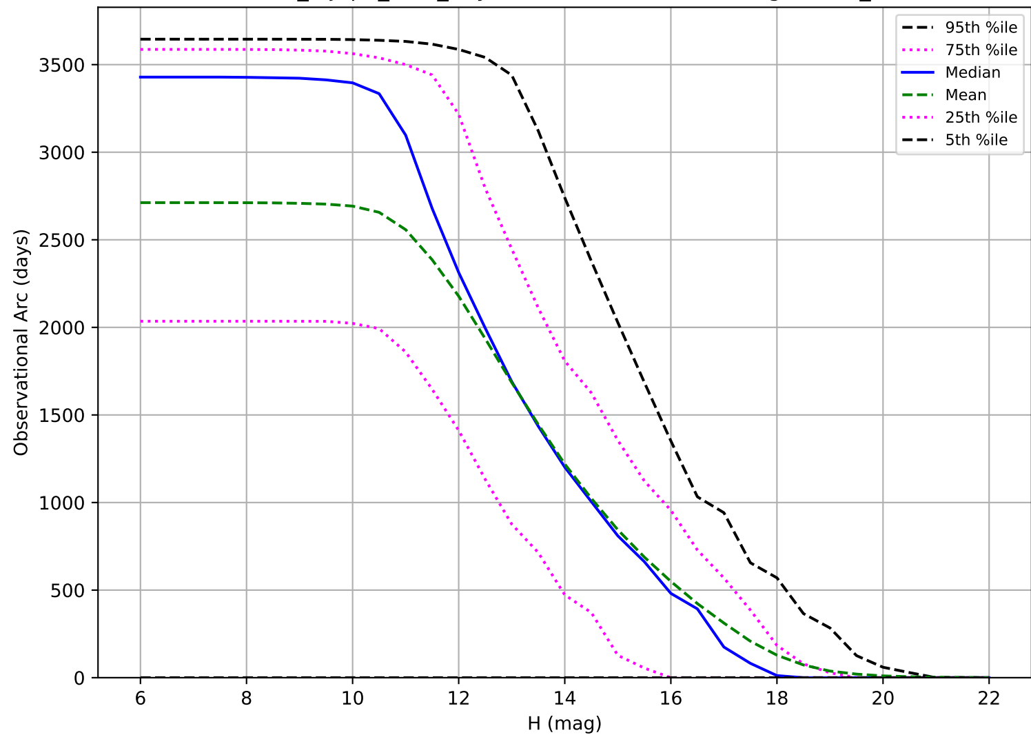
noroll_mjdp0_v3.4_10yrs: Observational Arc Length OCC_r5
