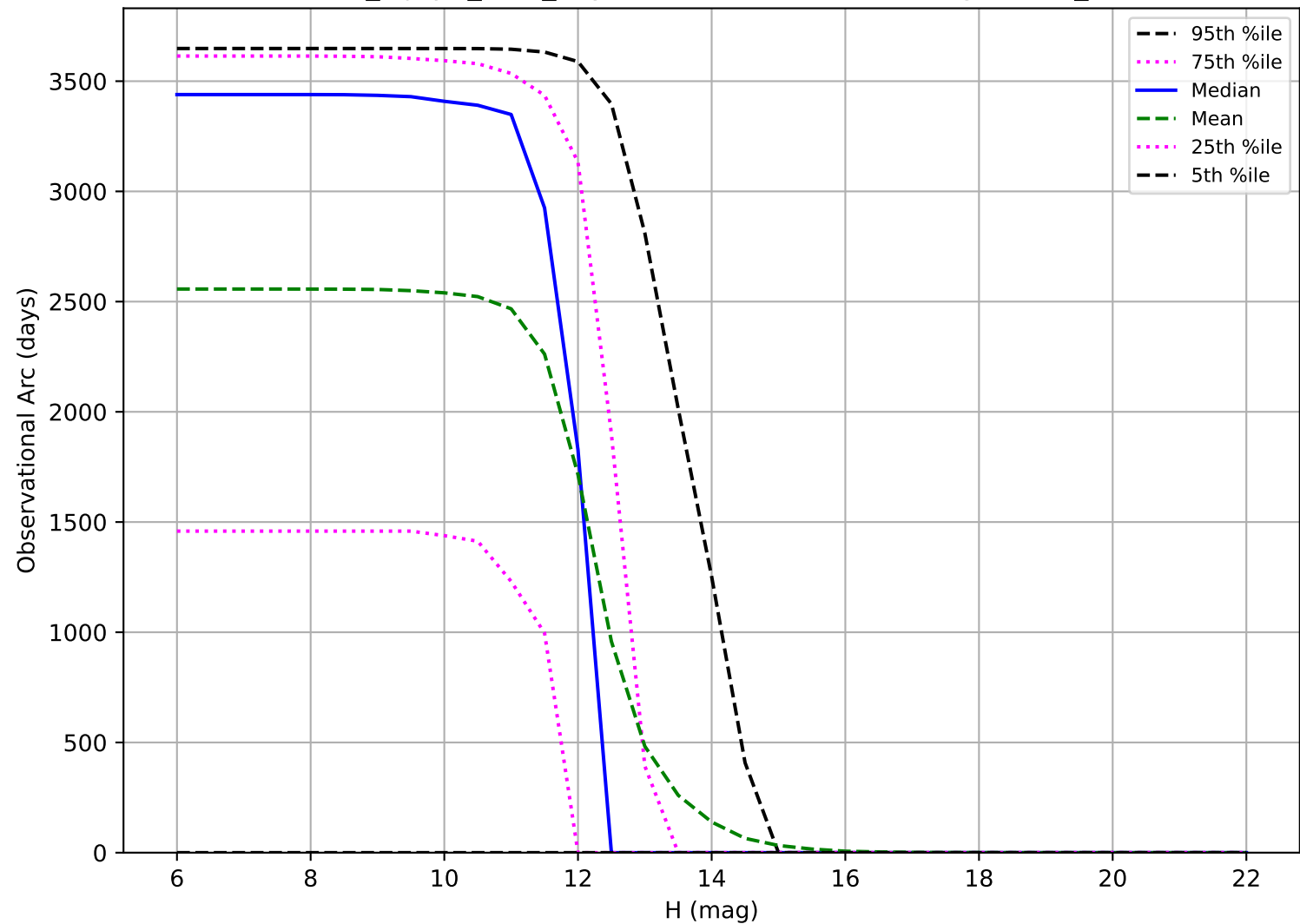
noroll_mjdp0_v3.4_10yrs: Observational Arc Length OCC_r20
