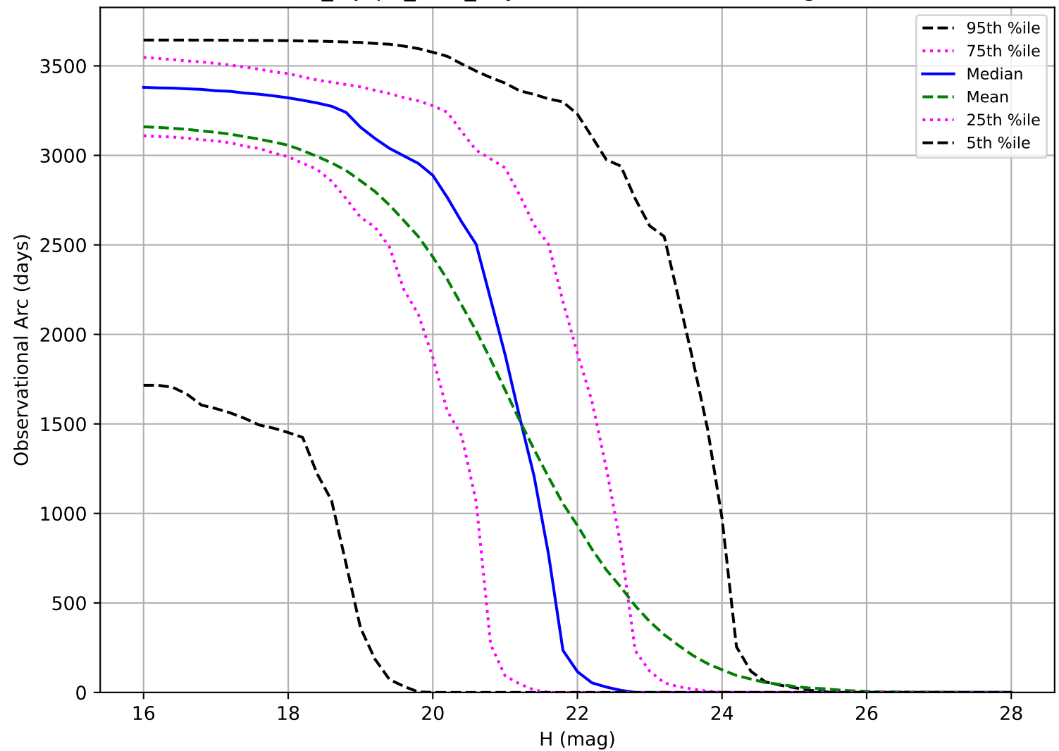
noroll_mjdp0_v3.4_10yrs: Observational Arc Length NEO
