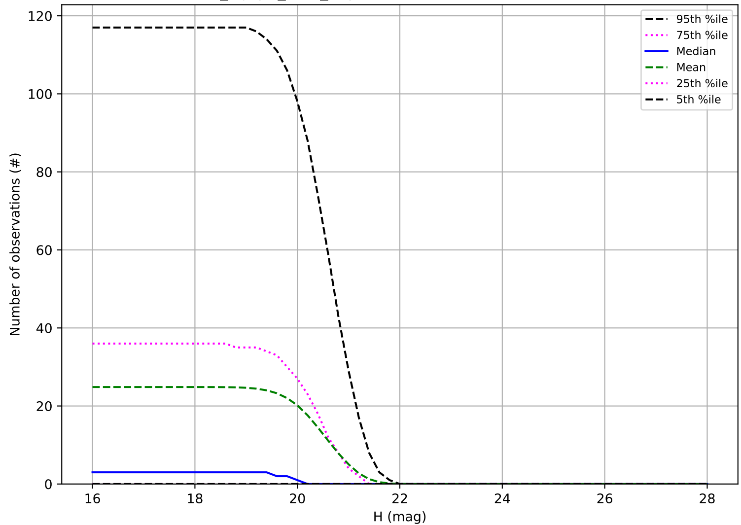
noroll_mjdp0_v3.4_10yrs: Number of observations Vatira
