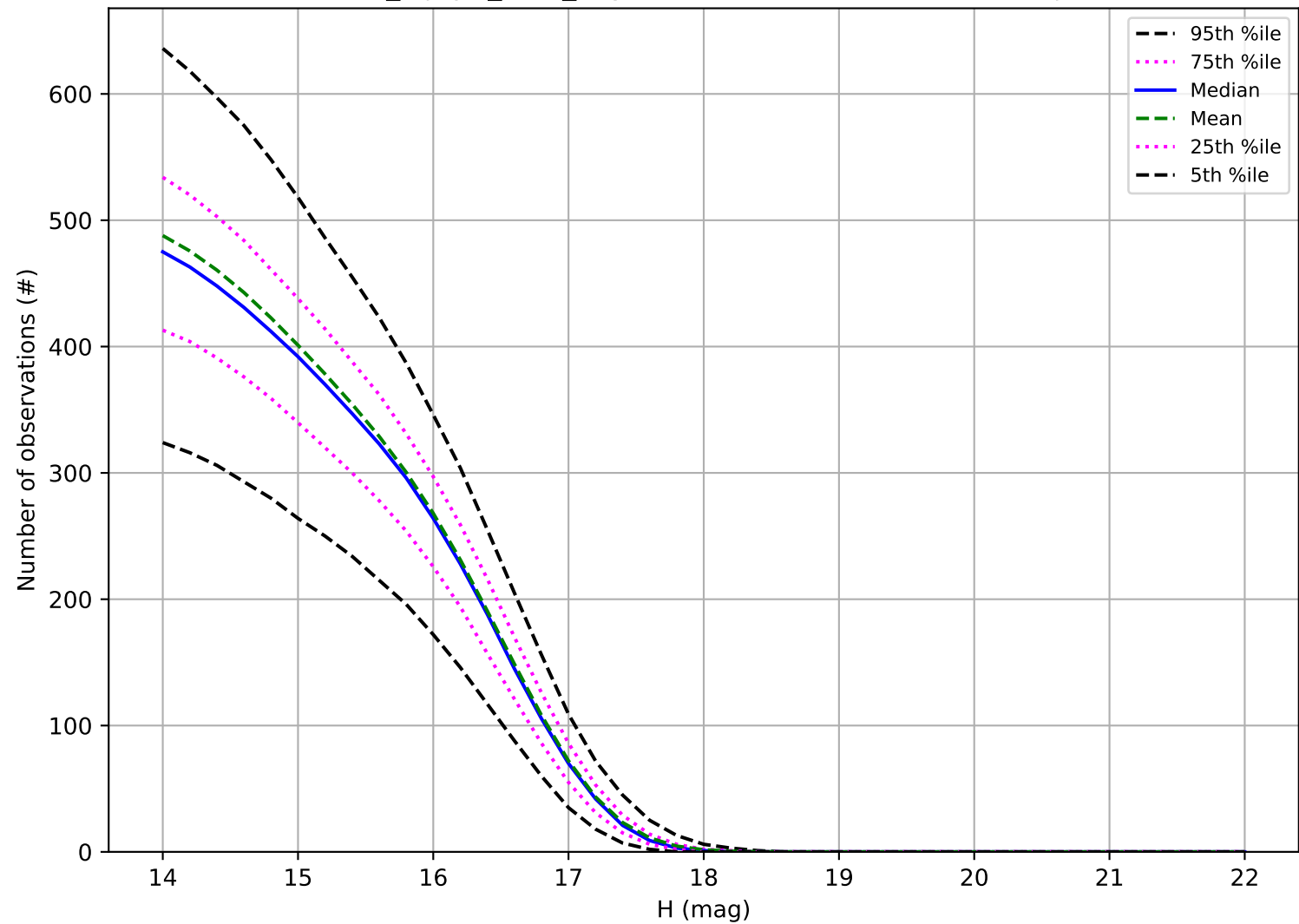
noroll_mjdp0_v3.4_10yrs: Number of observations Trojan
