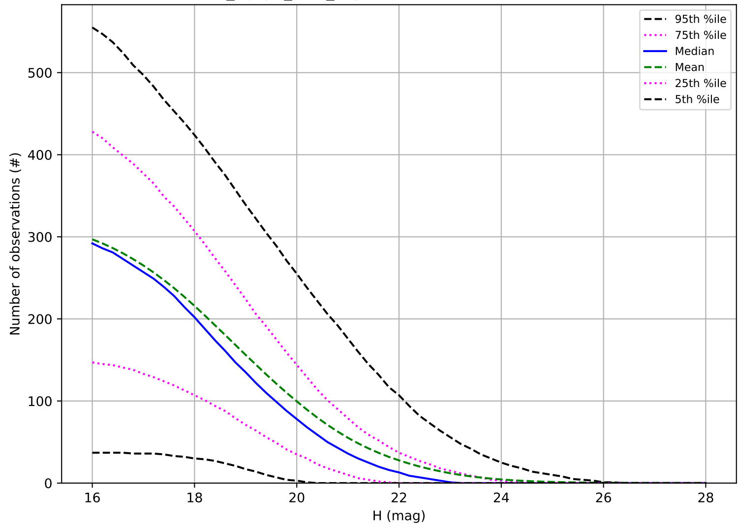
noroll_mjdp0_v3.4_10yrs: Number of observations PHA
