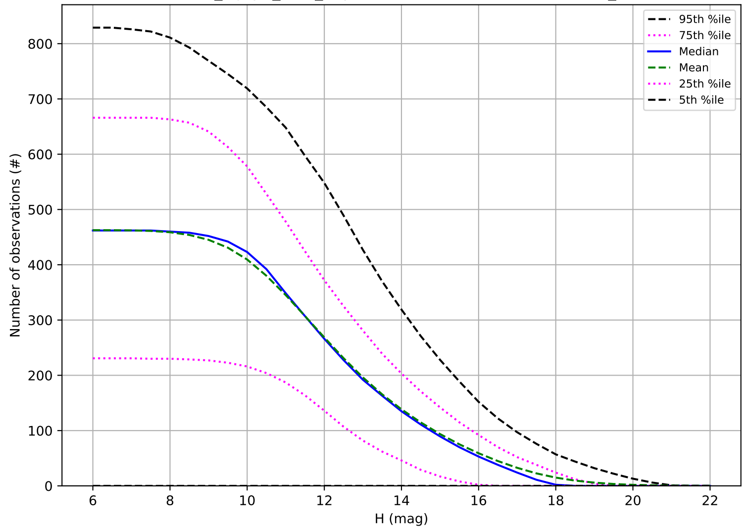
noroll_mjdp0_v3.4_10yrs: Number of observations OCC_r5
