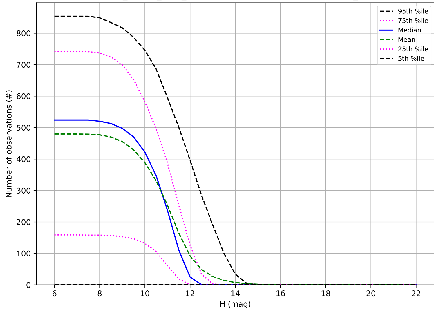
noroll_mjdp0_v3.4_10yrs: Number of observations OCC_r20
