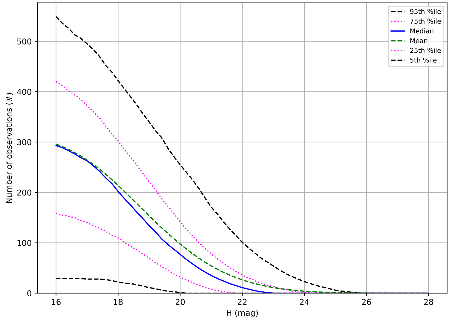
noroll_mjdp0_v3.4_10yrs: Number of observations NEO
