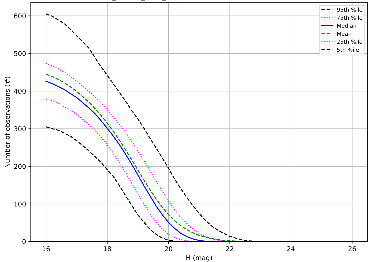
noroll_mjdp0_v3.4_10yrs: Number of observations MBA
