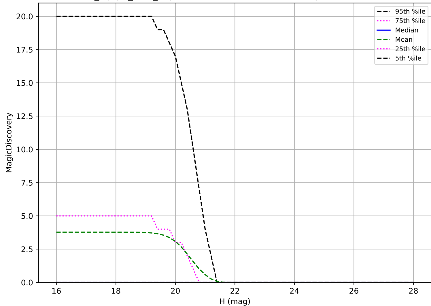
noroll_mjdp0_v3.4_10yrs: Vatra 6 detections in 60 nights detection loss
