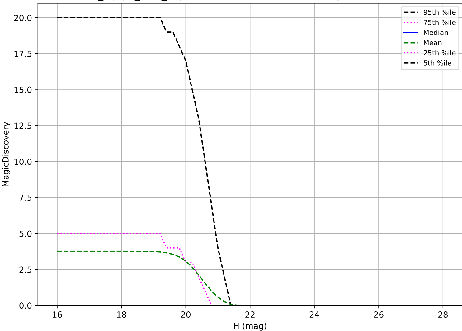
noroll_mjdp0_v3.4_10yrs: Vatira 6 detections in 60 nights detection loss
