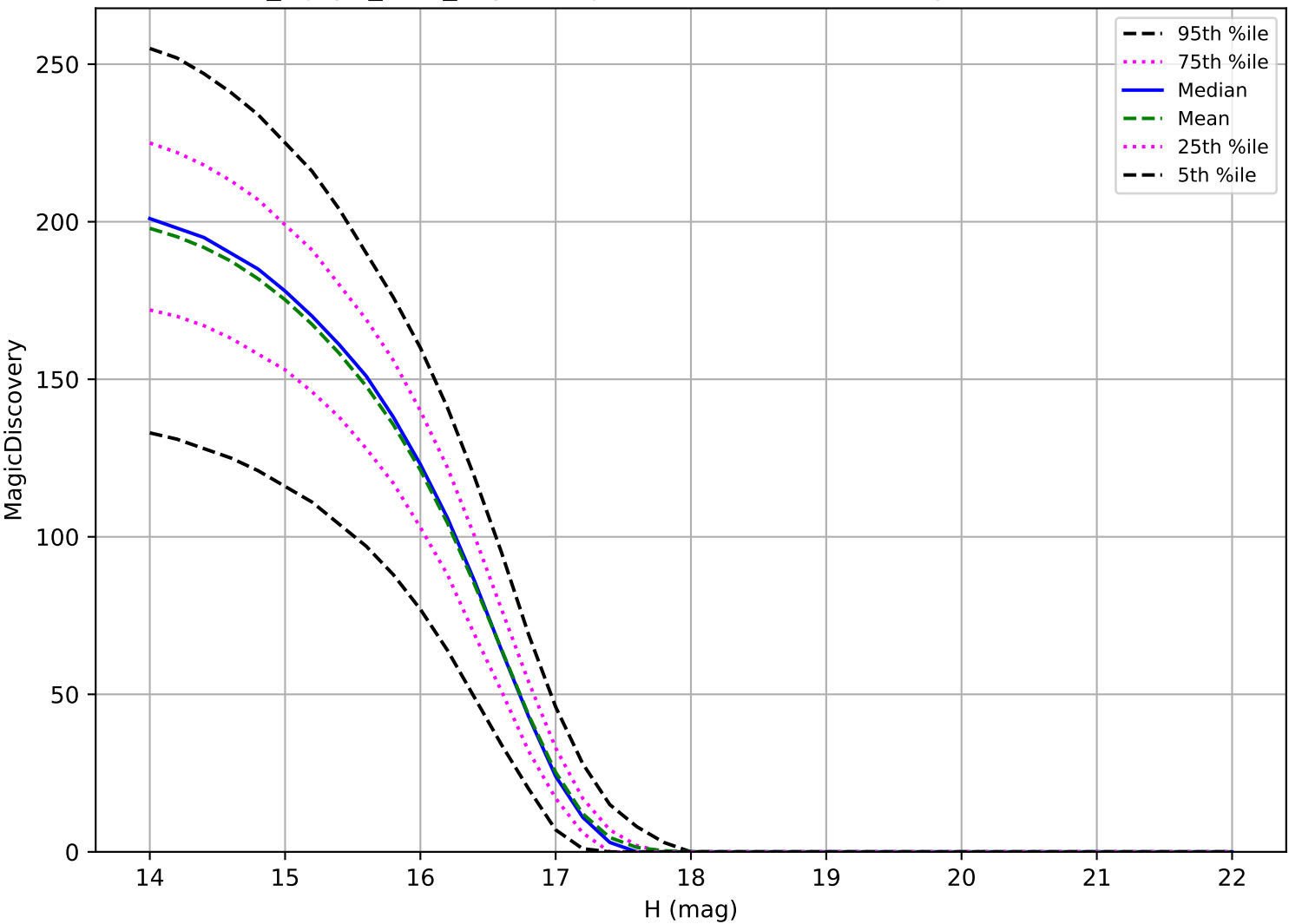
noroll_mjdp0_v3.4_10yrs: Trojan 6 detections in 60 nights detection loss
