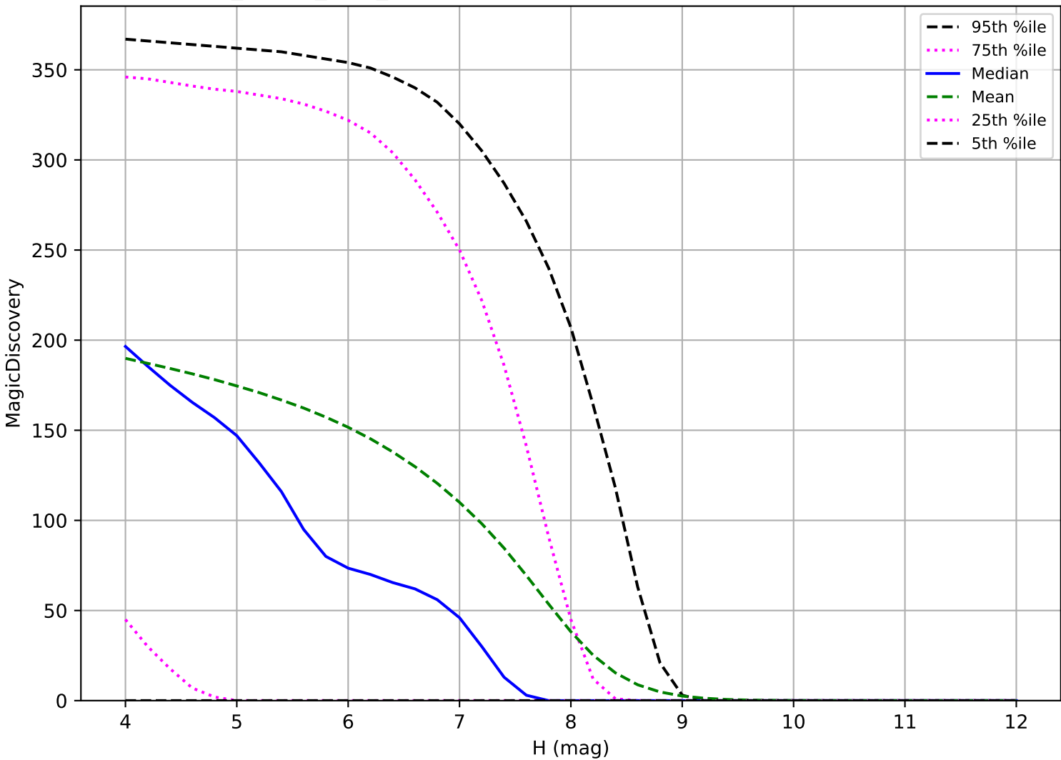
noroll_mjdp0_v3.4_10yrs: TNO 6 detections in 60 nights detection loss
