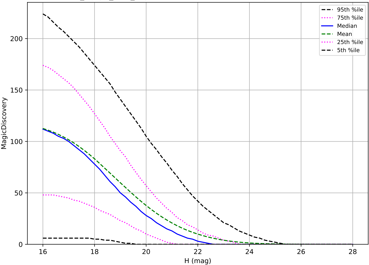
noroll_mjdp0_v3.4_10yrs: PHA 6 detections in 60 nights detection loss
