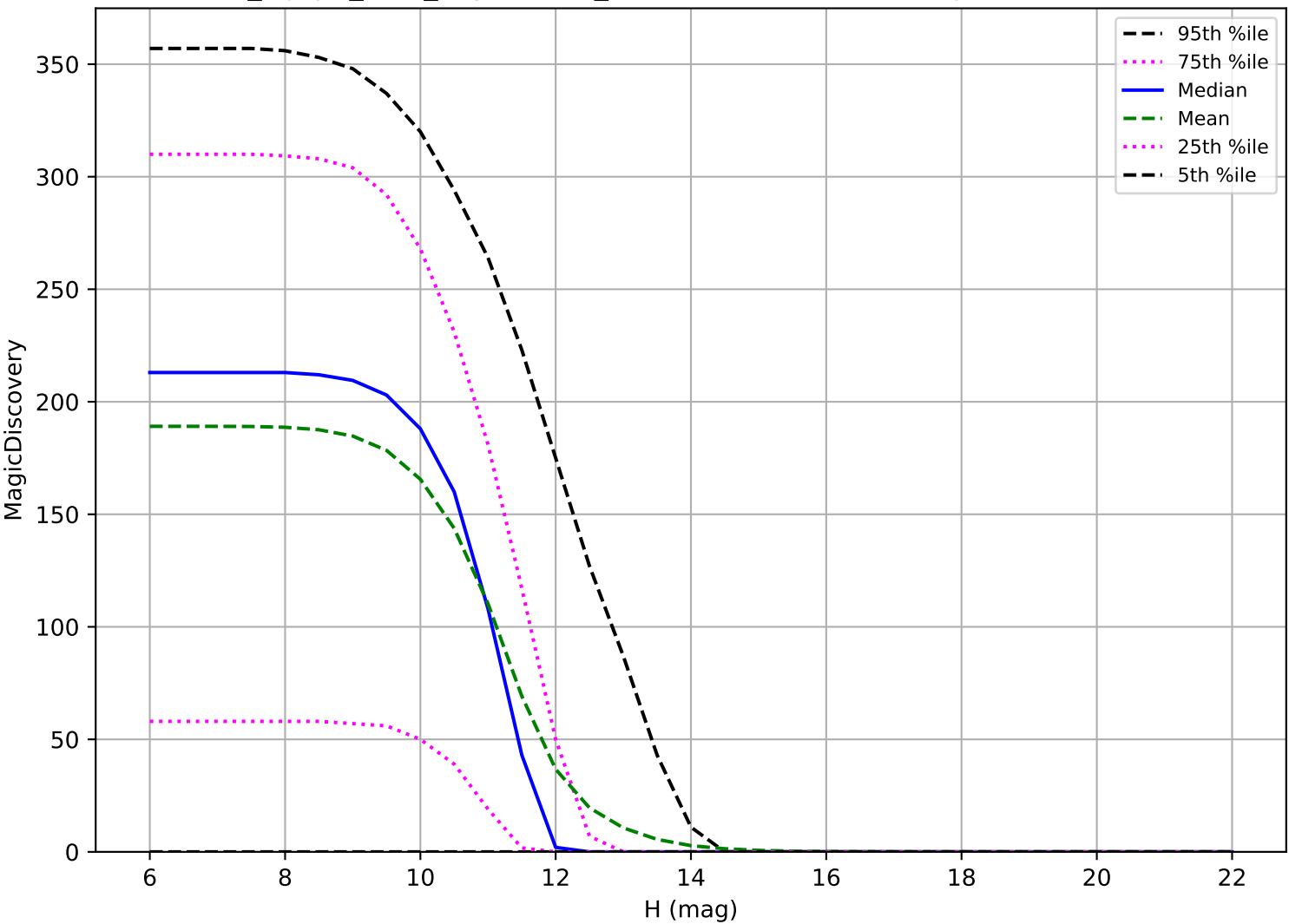
noroll_mjdp0_v3.4_10yrs: OCC_r20 6 detections in 60 nights detection loss
