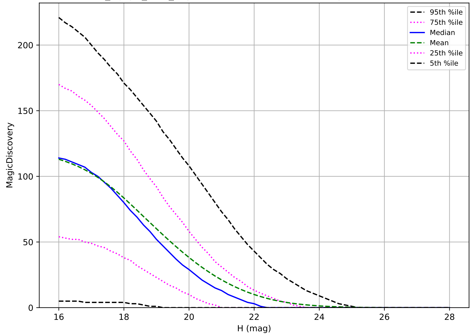
noroll_mjdp0_v3.4_10yrs: NEO 6 detections in 60 nights detection loss
