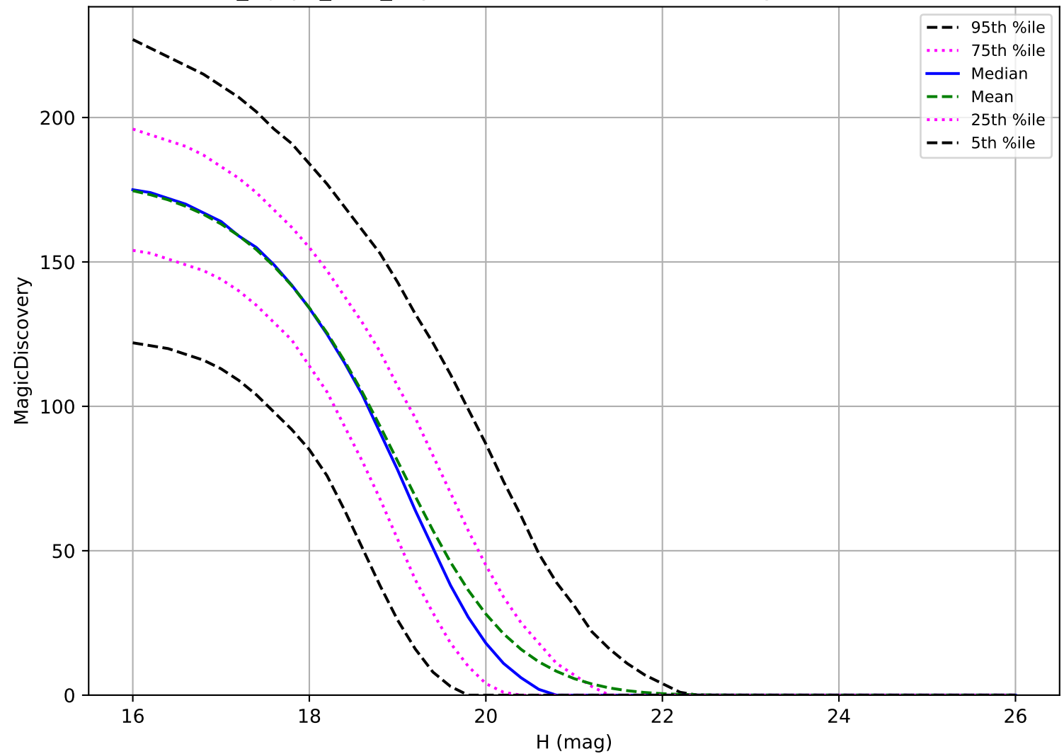
noroll_mjdp0_v3.4_10yrs: MBA 6 detections in 60 nights detection loss
