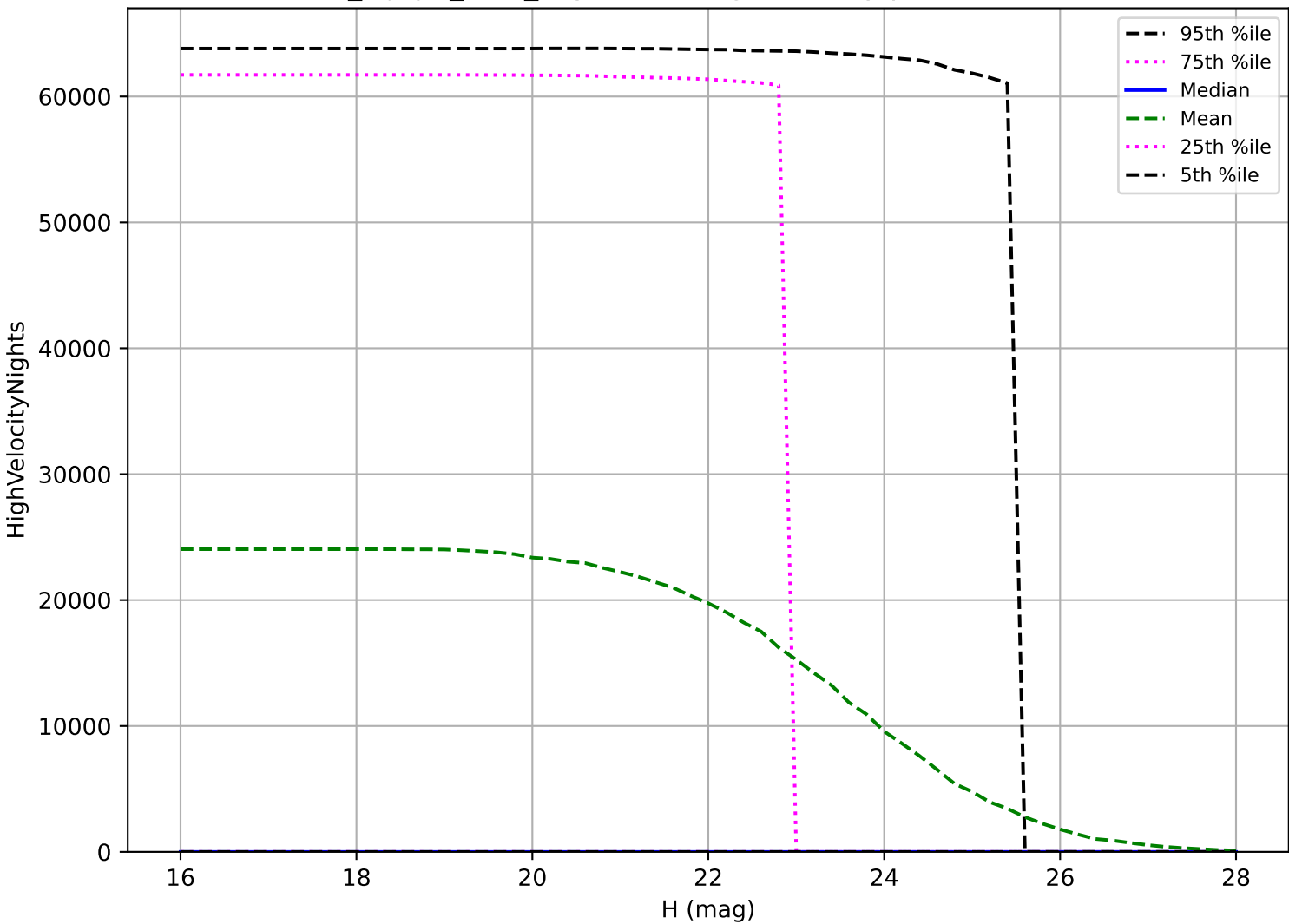
noroll_mjdp0_v3.4_10yrs: PHA High velocity pair detection loss
