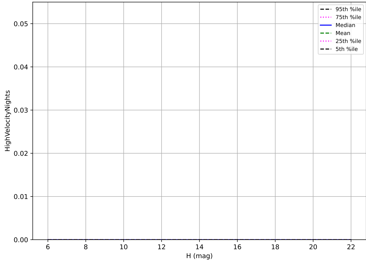
noroll_mjdp0_v3.4_10yrs: OCC_r5 High velocity pair detection loss
