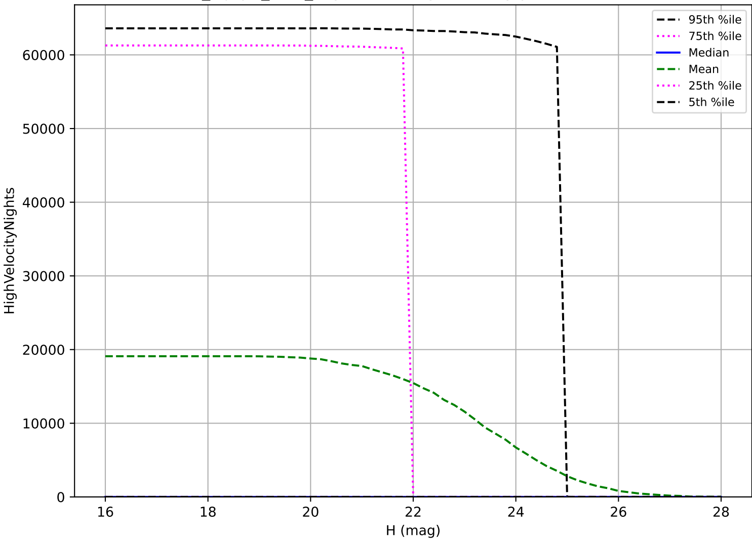
noroll_mjdp0_v3.4_10yrs: NEO High velocity pair detection loss
