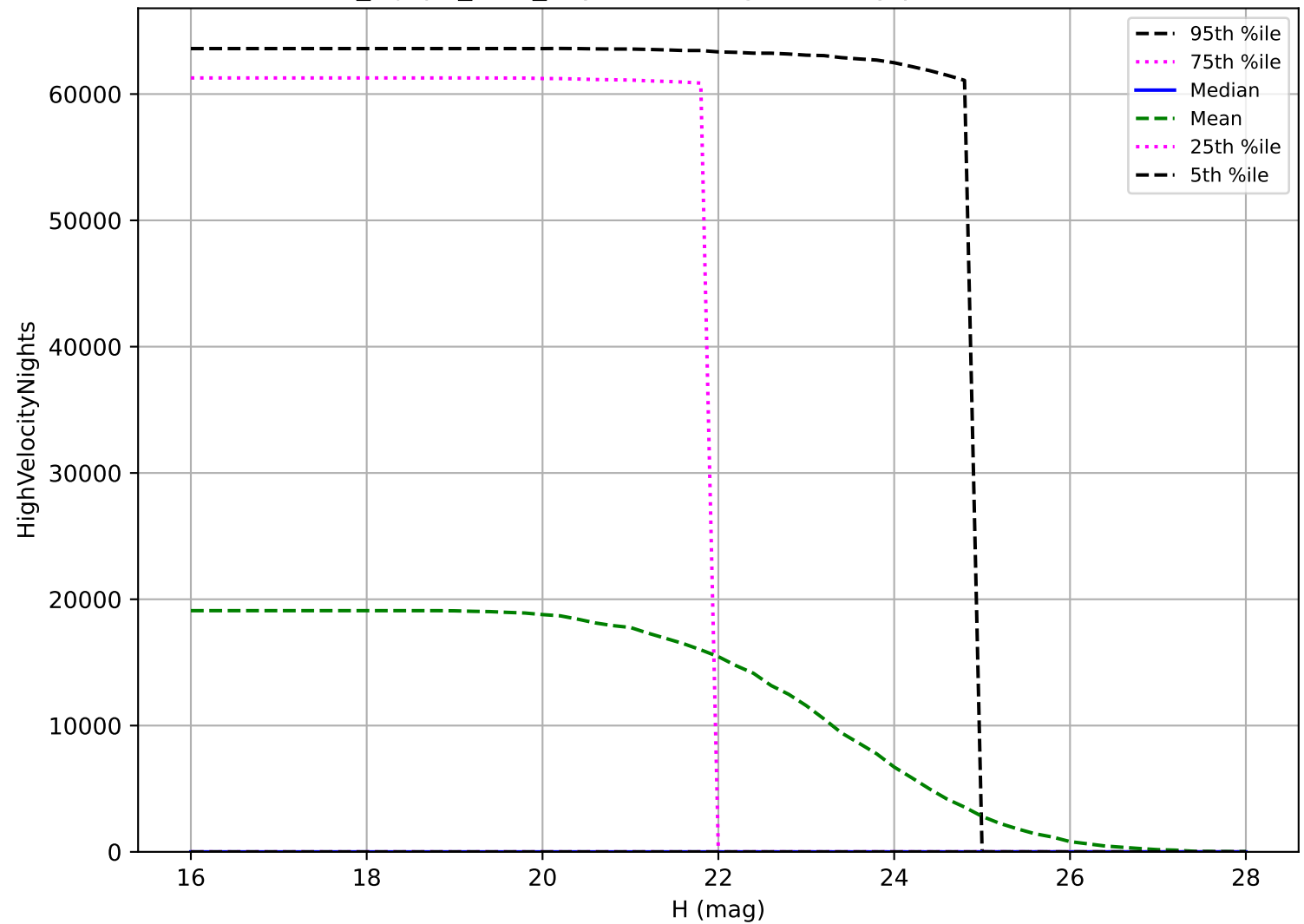
noroll_mjdp0_v3.4_10yrs: NEO High velocity pair detection loss
