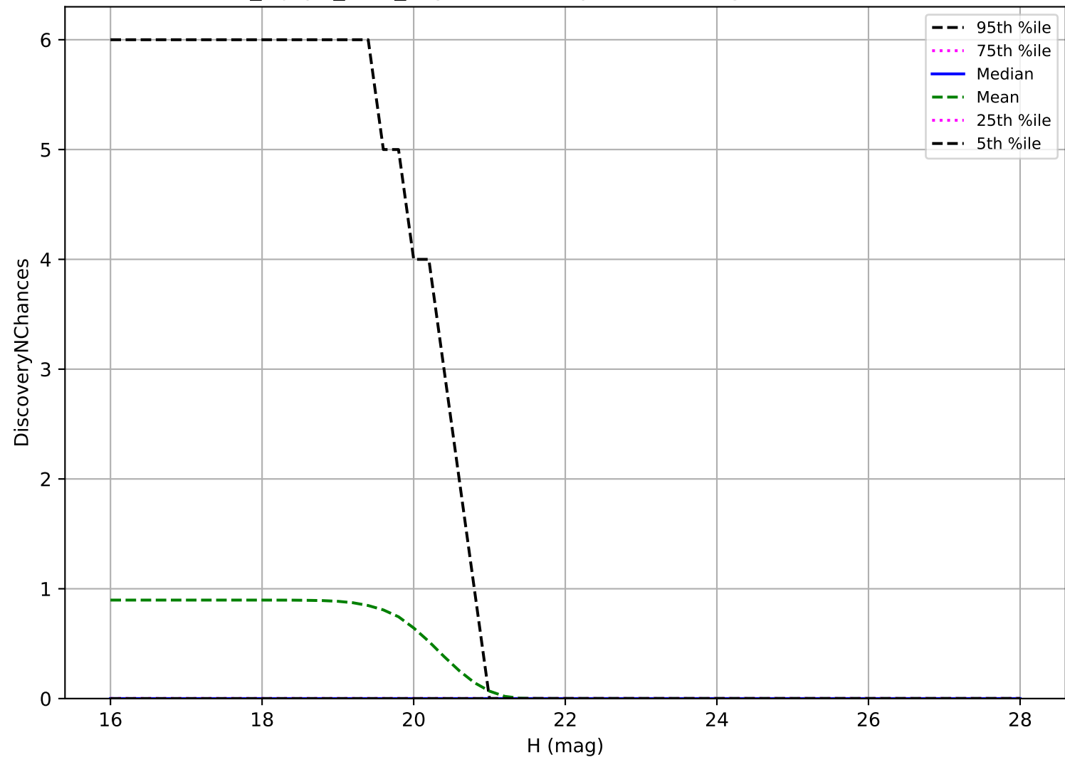
noroll_mjdp0_v3.4_10yrs: Vatira 3 pairs in 15 nights detection loss
