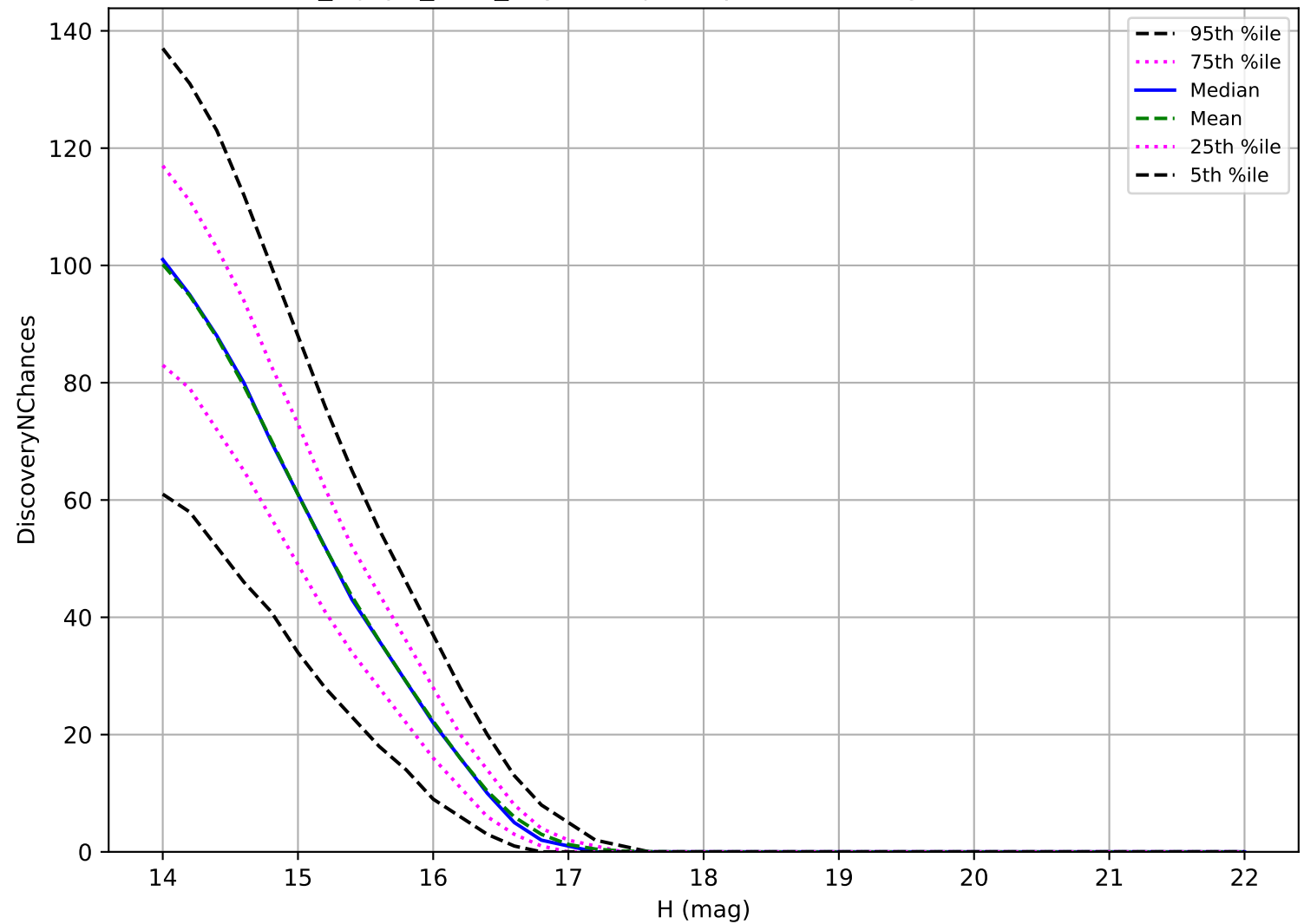
noroll_mjdp0_v3.4_10yrs: Trojan 3 pairs in 15 nights detection loss
