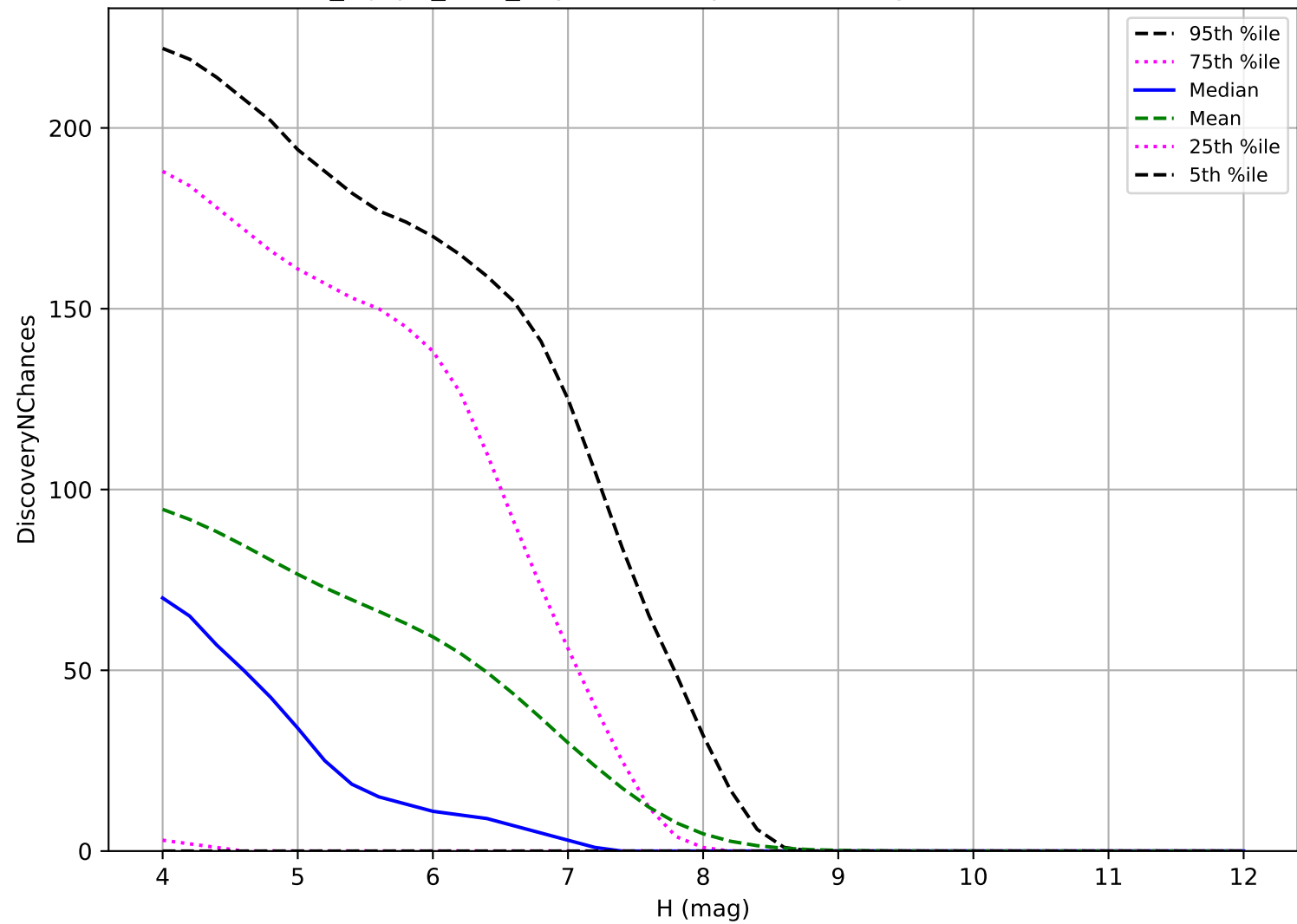
noroll_mjdp0_v3.4_10yrs: TNO 3 pairs in 15 nights detection loss
