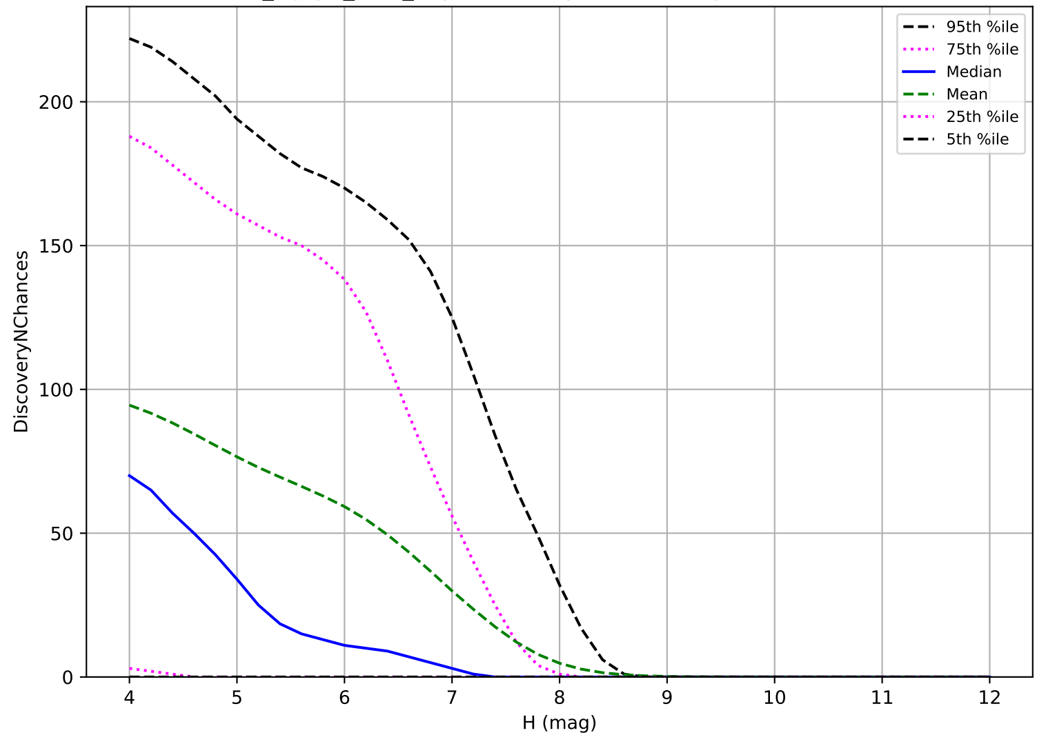
noroll_mjdp0_v3.4_10yrs: TNO 3 pairs in 15 nights detection loss
