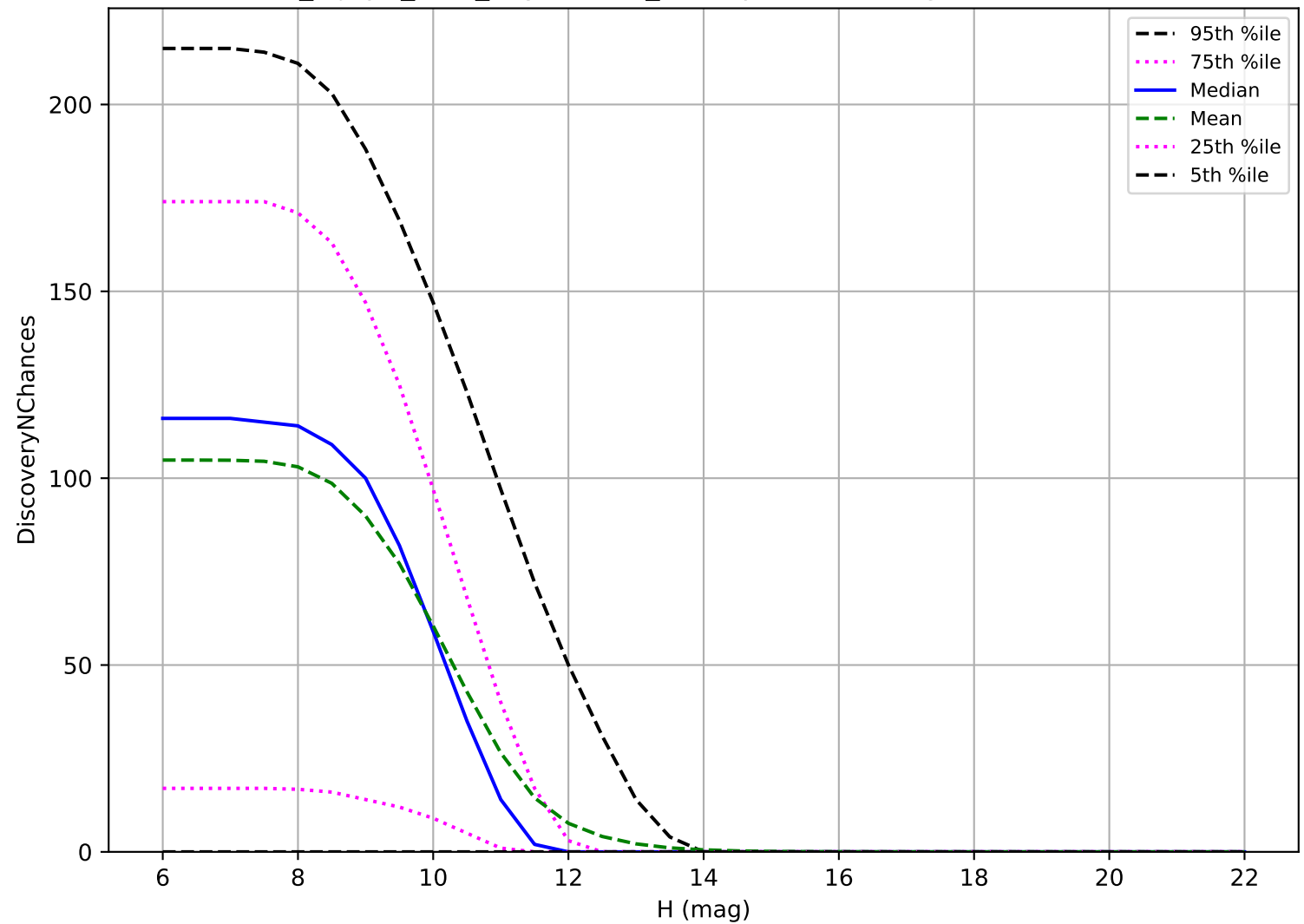
noroll_mjdp0_v3.4_10yrs: OCC_r20 3 pairs in 15 nights detection loss
